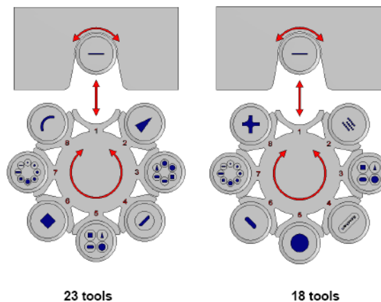
Tooling sample Multipunch
